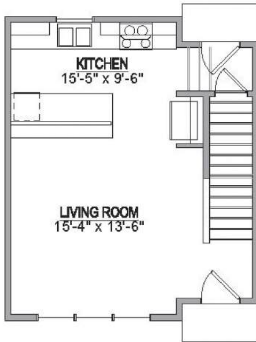
1st Floor
